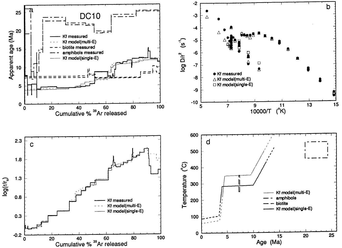
Fig. 18. (a) DC10 K-feldspar (bold line), biotite (short dashed) and amphibole (dot dashed) age spectra, (b) K-feldspar Arrhenius plot, (c) K-feldspar \log(\tau/r_0) plot, (d) cooling history; the corresponding K-feldspar model age spectra are the light lines on Figure 18a. See Figure 15 for details.
