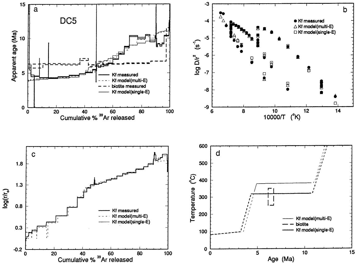
Fig. 17. (a) DC5 K-feldspar (bold line) and biotite (short dashed) age spectra, (b) K-feldspar Arrhenius plot, (c) K-feldspar \log(\tau/r_0) plot, (d) cooling history; the corresponding K-feldspar model age spectra are the light lines on Figure 17a. See Figure 15 for details.
