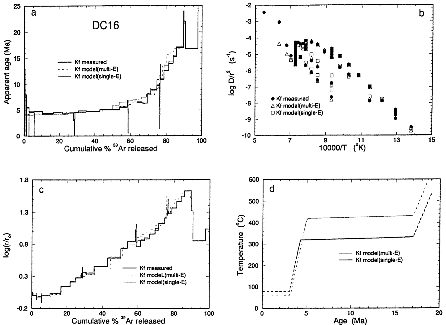
Fig. 19. DC16 K-feldspar (a) age spectrum, (b) Arrhenius plot, (c) \log(\tau/\tau_0) plot, (d) cooling history; the corresponding K-feldspar model age spectra are the light lines on Figure 19a. See Figure 15 for details.
