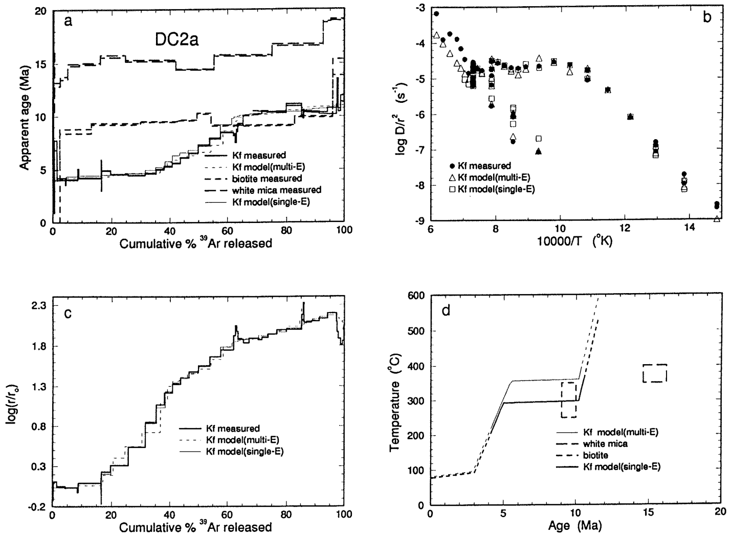
Fig. 16. (a) DC2a K-feldspar (bold line), biotite (short dashed) and white mica (dashed line) age spectra. (b) K-feldspar Arrhenius plot, (c) K-feldspar \log(r/r_0) plot, (d) cooling history; the corresponding K-feldspar model age spectra are the light lines on Figure 16a. See Figure 15 for details.
