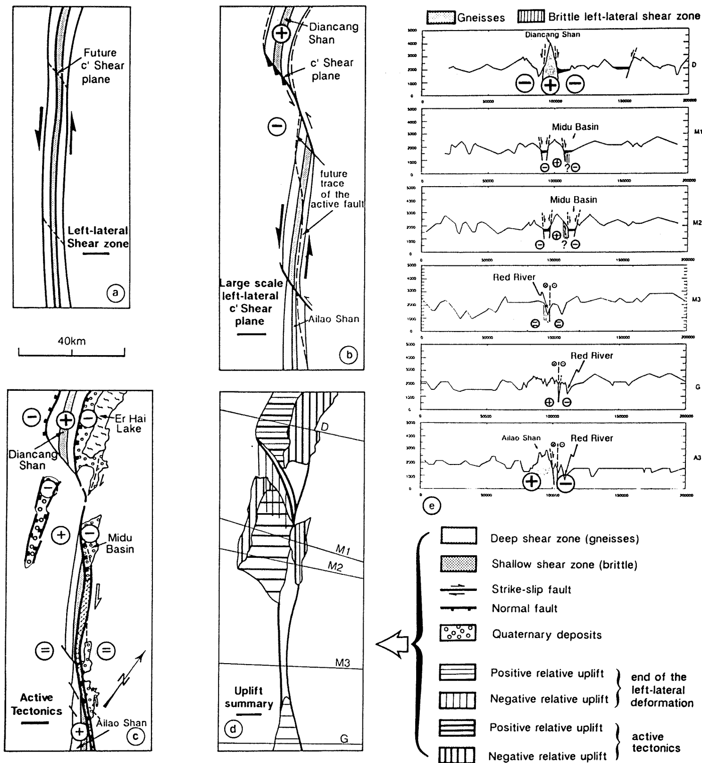
Fig. 24. Interpretative sketches of the structural evolution of the "Midu Gap". (a) Continuous left-lateral ductile shear zone. (b) Large-scale left-lateral C' shear planes affecting the shear zone. (c) Active faults: normal on each side of the Diancang Shan, right-lateral south of Midu, right-lateral and normal at the northern end of the Ailao Shan. (d) Qualitative summary of corresponding total uplift. The topographic sections DCS1, M1, M2, M3, and G are shown on Figure 24e. Section A3 is located farther south near the town of Gasa. Metamorphic rocks outcrop where the total uplift is greater. (e) Qualitative estimation of recent uplift along sections across the Red River fault. Sections are located on Figure 24d. Topography from Chinese 1/100,000 scale topographic maps and ONC maps. The vertical exaggeration is 10x.
