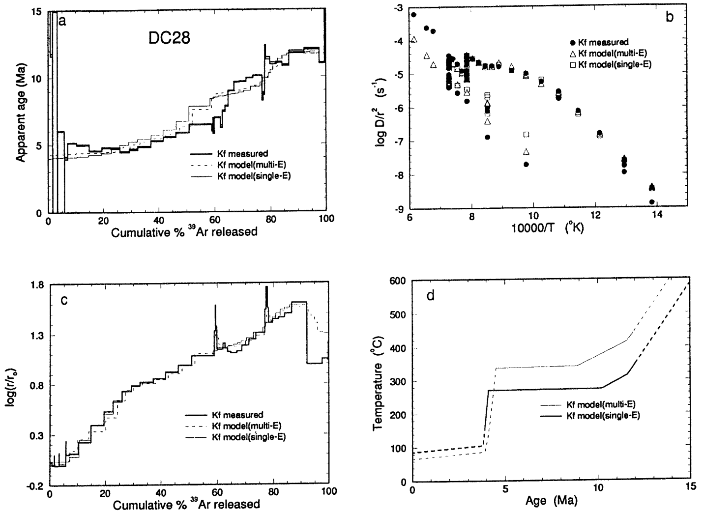
Fig. 20. DC28 K-feldspar (a) age spectrum, (b) Arrhenius plot, (c) \log(\tau/\tau_0) plot, (d) cooling history; the corresponding K-feldspar model age spectra are the light lines on Figure 20a. See Figure 15 for details.
