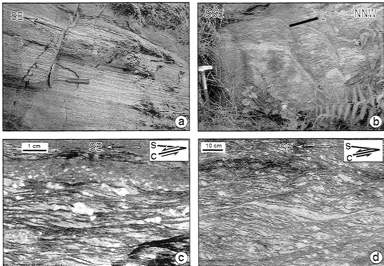
Figure 7. Field observations along BatXat section (section A, Figure 6). (a) Well-banded mylonites at site A8; foliation strikes N145^\circ (view from above, hammer gives scale). (b) Steep foliation ( N159^\circ , 83^\circ W ) and sub-horizontal stretching lineation (pitch 18S ) at site A3 (hammer gives scale). (c) Polished slab of sample V106 showing left-lateral C/S structures at site A3 (view from above). (d) Late left-lateral C/S structures at site A3 (view from above).
