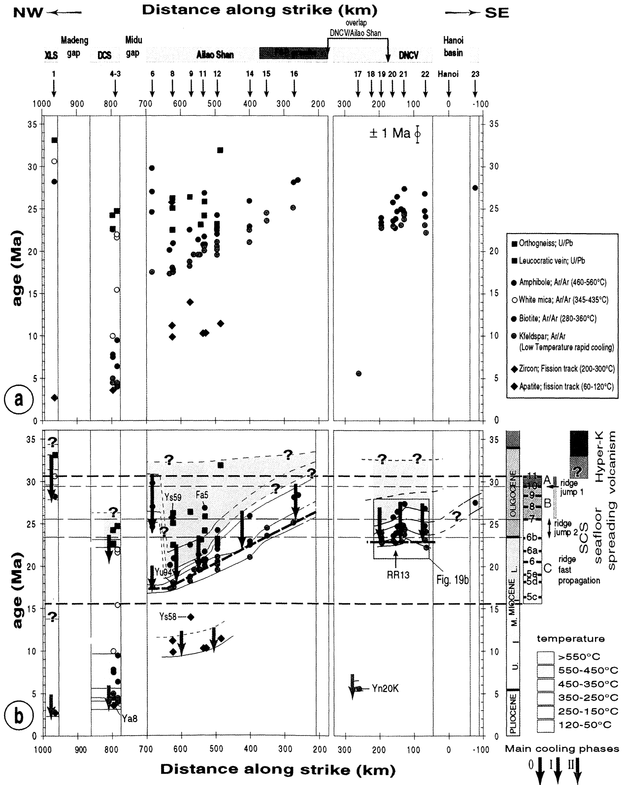
Plate 2. Summary of thermochronological data for entire ASRR. Same representation as for Figure 19. DayNuiConVoi and Ailao Shan ranges overlap near the China/Vietnam border. (a) All data (Table 7). Fission track results from Bergman et al. [1997] and S. Bergman (personal communication, 1998), and ^{40}\text{Ar}/^{39}\text{Ar} results are from Leloup et al. [1993], Chen et al. [1993], Harrison et al. [1996], Wang et al. [1998], and this study, U-Pb results are from Schärer et al. [1990, 1994] and Zhang and Schärer [1999]. Uncertainties on most samples are much less than \pm 1 Ma (Table 7). Because of across-strike diachronous cooling in Ailao Shan, only data coming from <10 km from the range NE border are plotted. (b) Time/temperature domains deduced from Plate 2a. Note the contrasted cooling histories in the four ranges of ASRR. SCS seafloor spreading timing is plotted on the right for comparison.
