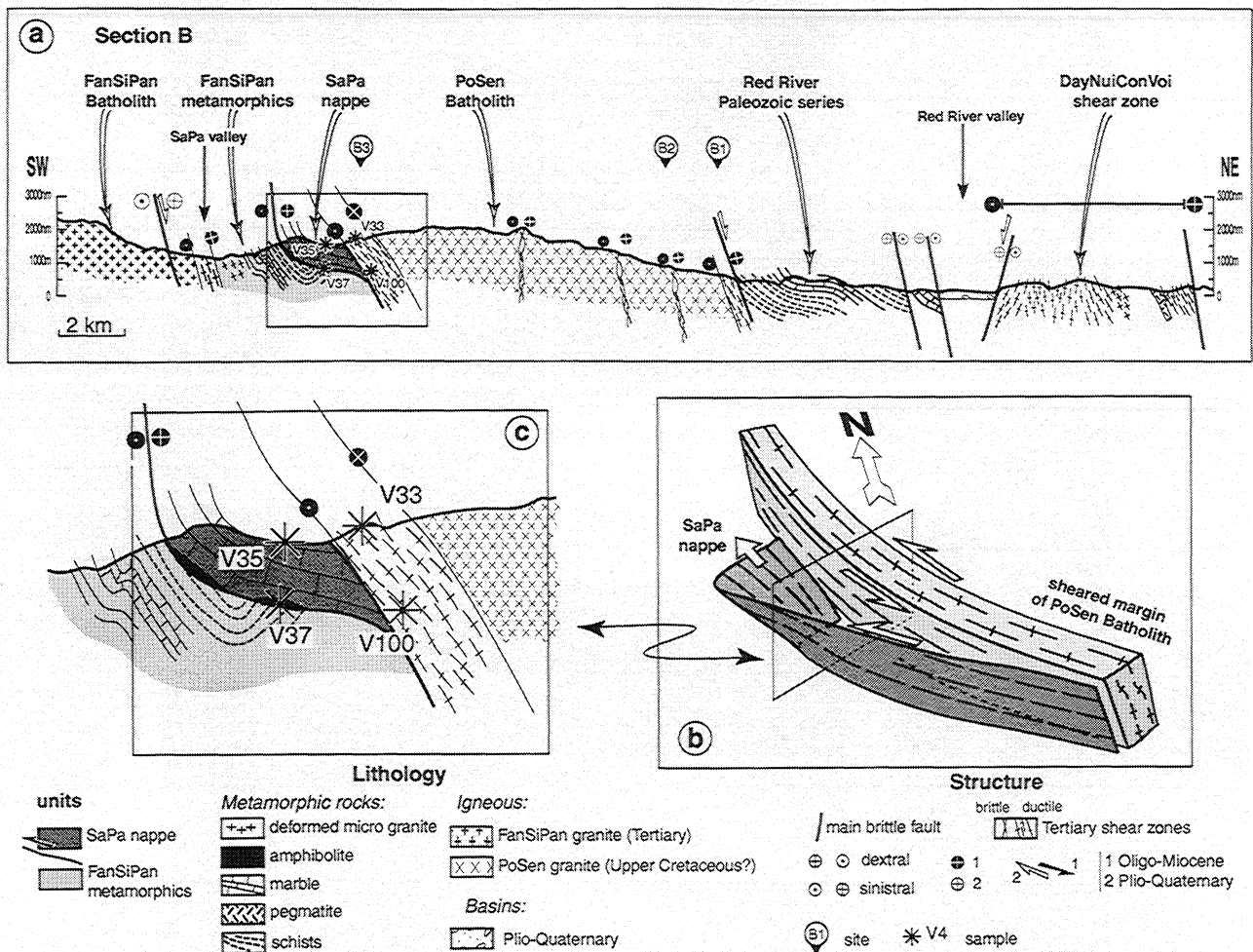
Figure 9. (a) LaoCay-Sapa cross section (section B, Figure 5). Drawn from geological map [ General Geological Directorate of Vietnam, 1978 ] and field work. (b) Schematic 3-D representation of SaPa nappe. See also Figures 8b and 8c. (c) Zoom of the SW border of the Posen granite and SaPa thrust.
