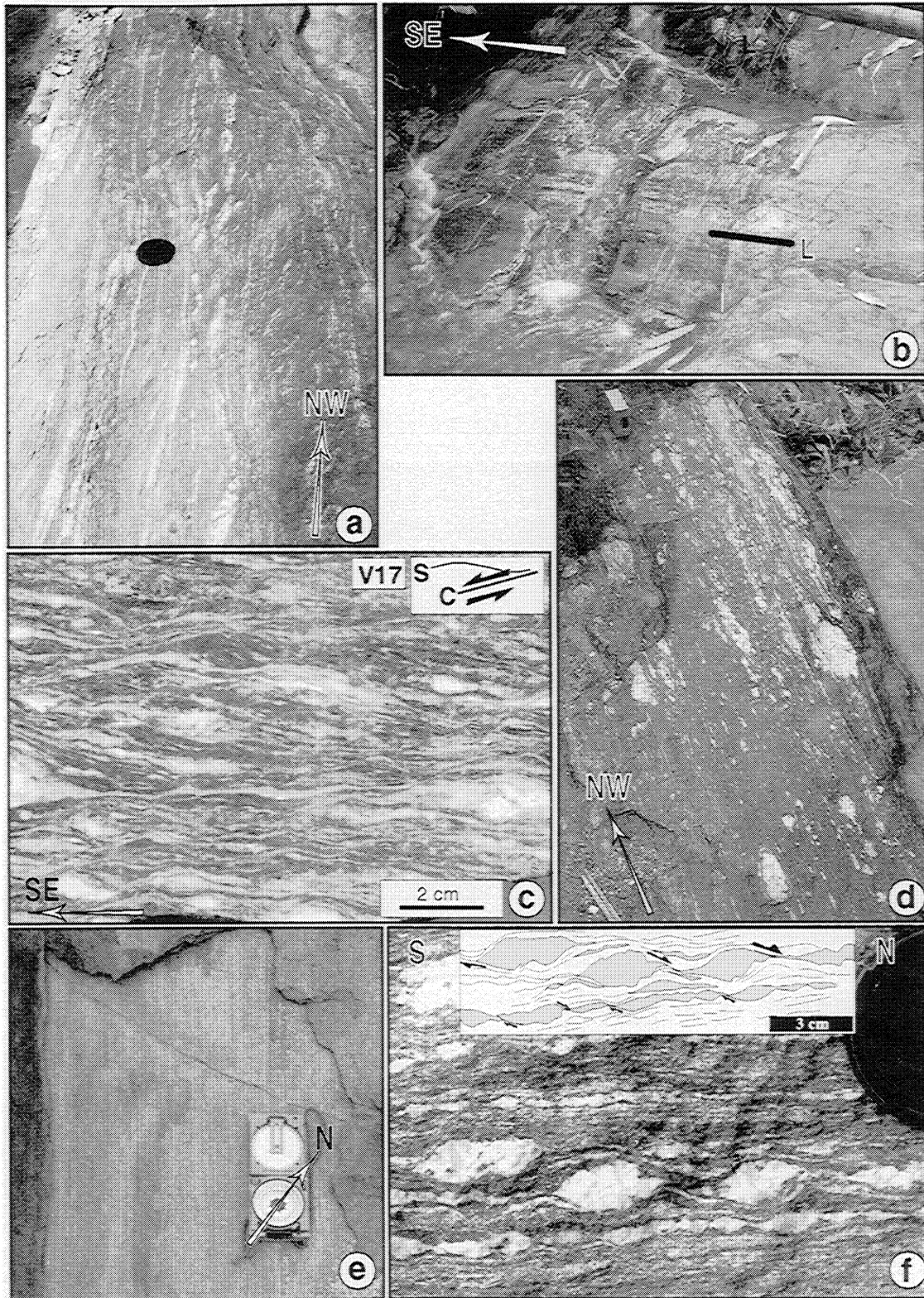
Figure 15. Structural field observations in DayNuiConVoi range. Sites located on Figures 4, 12 and 14a. (a) Banded steep mylonites at site D6, foliation strikes N140^{\circ} (view from above, lens cap gives scale). (b) Steep foliation ( N147^{\circ}, 78^{\circ}\text{NE} ) and subhorizontal stretching lineation (pitch 18^{\circ}\text{S} ) at site D5. (c) Polished slab of sample V17 (site D7) showing left-lateral C/S structures (view from above). (d) High-temperature foliation (site D5) typical of DayNuiConVoi range striking N150^{\circ} (view from above). (e) Flat foliation and N165^{\circ} trending stretching lineation at site G (compass gives scale). (f) Shear criteria indicating top to the north shear at site G.
