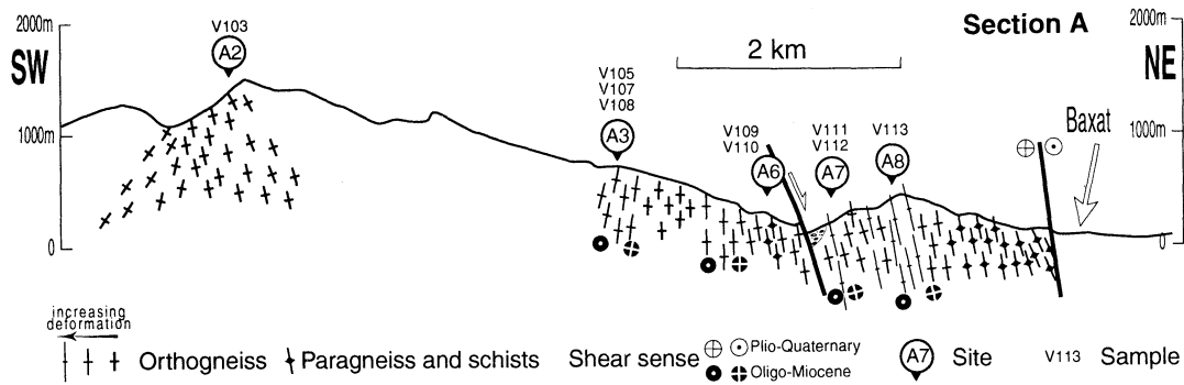
Figure 6. BatXat cross section (section A), located on Figure 5b, showing samples and sites discussed in text. Corresponding foliation and lineation attitudes are plotted on Figure 8a.
