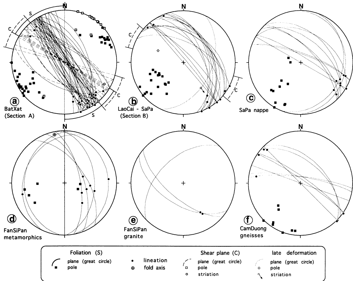
Figure 8. Structural data from FanSiPan range (Schmidt diagram lower hemisphere). (a) BatXat section (section A, Figures 5 and 6), 37 foliations, 34 lineations, and 12 shear planes (shaded). (b) LaoCai-Sapa section (sites B1 to B4, Figures 5 and 9a), 19 foliations and 13 lineations. (c) Sapa thrust (Sapa nappe, Figures 5 and 9a), 11 foliations, and 8 lineations. (d) FanSiPan metamorphics (FSP metamorphics, Figures 5 and 9a), 9 foliations and 6 lineations. (e) FanSiPan granite, 3 foliations and 2 lineations (Figure 5). (f) CamDuong area (Figure 5), 8 foliations and 7 lineations.
