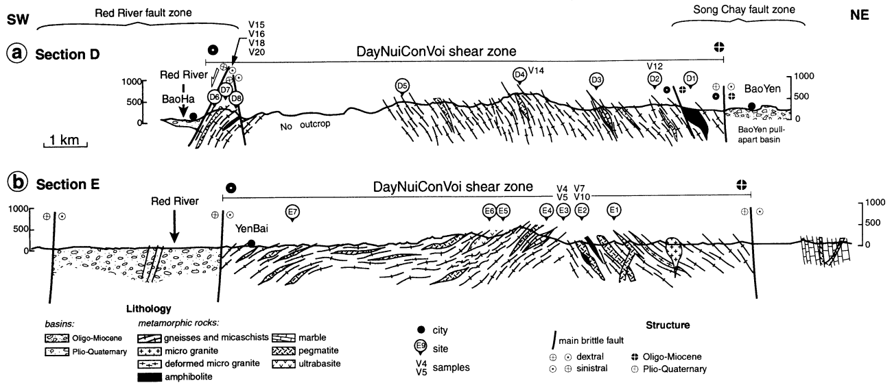
Figure 14. Cross sections of DayNuiConVoi metamorphic range. Sections are located on Figure 12. (a) BaoYen-BaoHa section (section D, Figures 13c, 15a-d and 16. (b) YenBai-YenBinh-TanHuong section (section E, Figure 13d).
