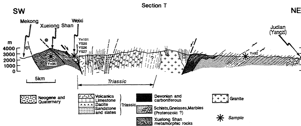
Figure 2. Section of northwestern ASRR across XueLong Shan range (see location on Figure 1). Simplified from Figure 9b of Leloup et al. [1995] with permission of Elsevier Science.
