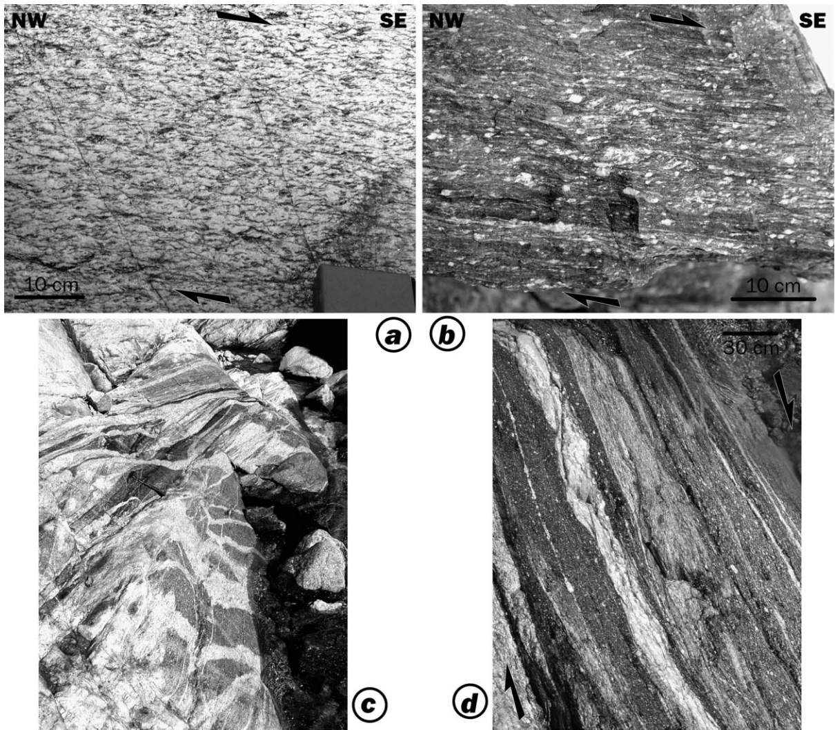
Fig. 4. Characters of deformation in gneisses and mylonites. a: C/S leucogranitic gneiss (section 4, Fig. 2). b: Dextrally sheared mylonites close to range front (section 3, Fig. 2). c: Several generations of synkinematic leucocratic veins intruding biotite-bearing gneisses (section 4, Fig. 2). d: Example of dextrally sheared leucocratic vein and gneisses (section 4, Fig. 2).
