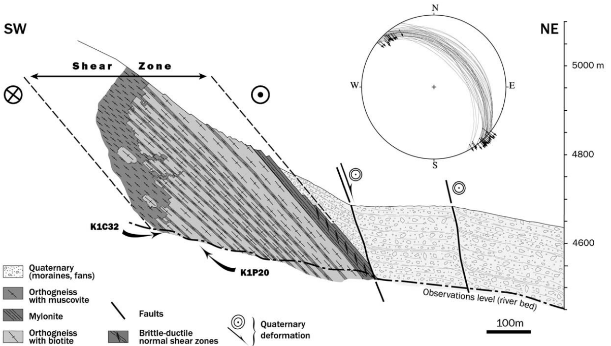
Fig. 3. Typical section of mylonites and gneisses west of Shiquanhe (section 4, Fig. 2); Schmid diagram (lower hemisphere) shows geometry of foliations (great circles) and of lineations (arrows). Samples dated with U/Pb techniques (Fig. 5) are located.
