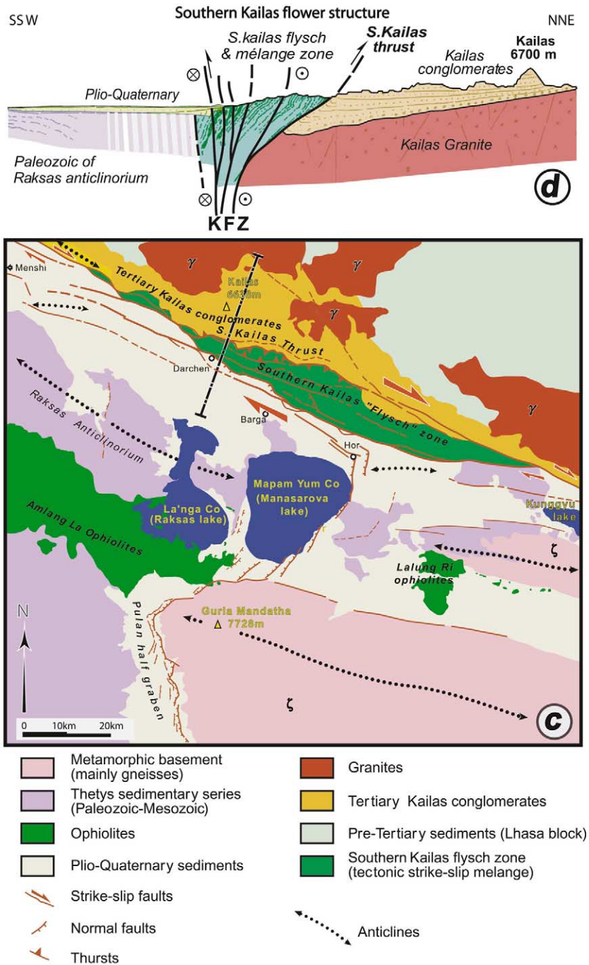
Fig. 6. Geometry of southern KFZ in Kailas region. a: Part of Landsat 7 image. b: Fault trace geometry, after field observations, geological maps [11,23,34] and satellite image interpretation, on Landsat image. c: Corresponding structural sketch. d: Interpretation of Gansser [23] synthetic section of the Kailas Range; approximative location of section shown by black hatched line on structural sketch.
