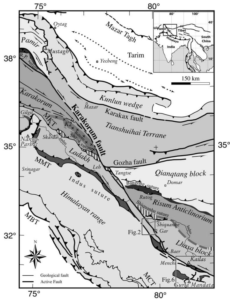
Fig. 1. Large-scale sketch map of KFZ and adjacent units. Inset shows location in large-scale Asian tectonic framework. Dark-gray tones outline the Indus-Zangbo, and the Bangong-Nujiang/Rushan-Pshart (R.P.) suture zones. Hatched tones correspond to Shiquanhe and Shyok suture zones.
