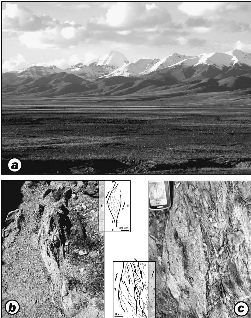
Fig. 7. a: View of Kailas-Ponri Range. Kailas is the rounded snowy mountain in the middle; note horizontal bedding in molasses beds below the summit. b,c: Typical characters of brittle-ductile deformation in southern Kailas flysch zone (vertical slivers and cleavage, sheared slivers and C/S shear planes); both images show structures on horizontal planes (oblique view towards west on b; view from above on c).
