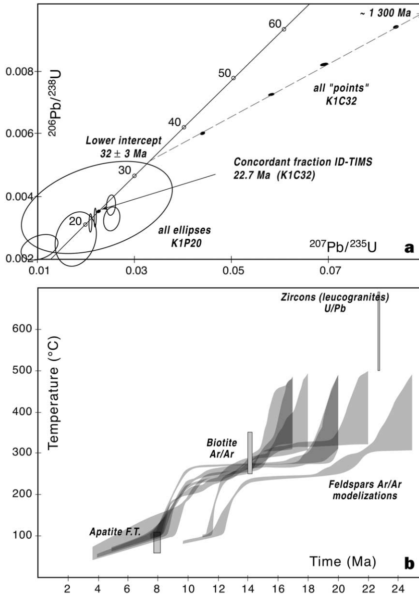
Fig. 5. Age results on gneisses and mylonites from sections 1–5 (Fig. 2). a: Concordia diagram showing U/Pb results on leucogranites from section 4 (Fig. 3). Small black ellipses show results obtained on different zircon fractions from sample K1C32 ( 2\sigma error); large open ellipses show concordant zircon ages from microprobe dating (sample K1P20); both samples are located on Fig. 3. b: Summary of cooling histories deduced from Ar/Ar dating; grayed areas: results of K-feldspar modeling [21] within 2\sigma error (seven samples coming from sections 1–5). Results obtained for one biotite, U/Pb zircon age of leucogranites (this study), and one apatite fission track age [22] are also shown for comparison.
