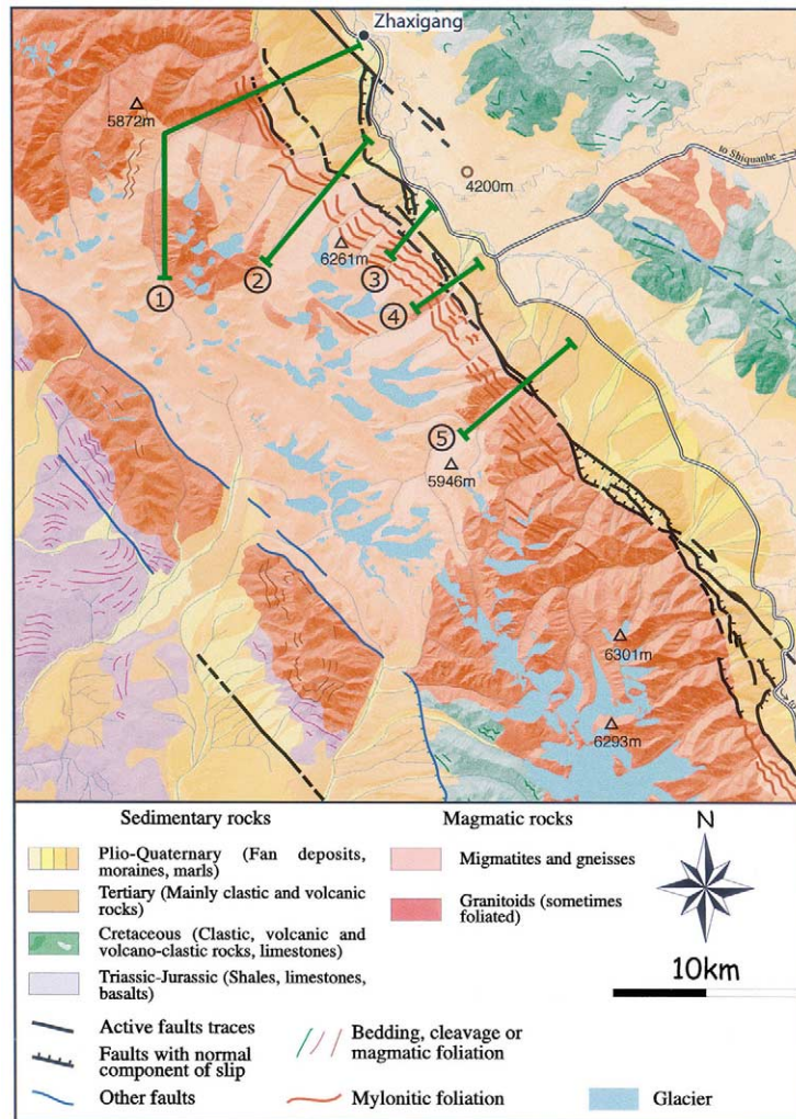
Fig. 2. Geological map of Ladakh-Karakorum Range between Zhaxigang and Gar, west of Shiquanhe. Drawn from field observations and satellite (Landsat, Spot) image interpretation. Light shading outlines topography. Five sections studied in the field are shown by green lines. Section 6 is located \sim 40 km south, near Gar city.
