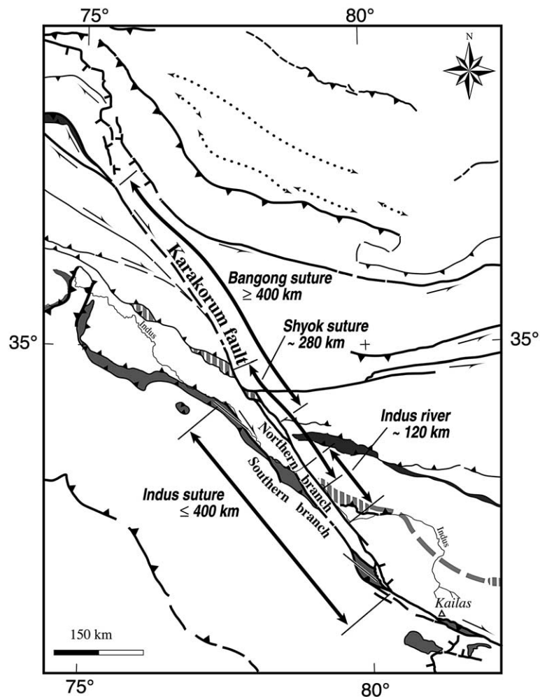
Fig. 8. Plausible offset values on the different branches of KFZ. See Fig. 1 for unit description, and text for discussion.
